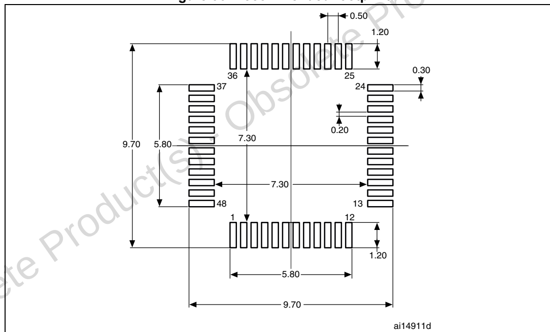
Figure 36. Recommended footprint
