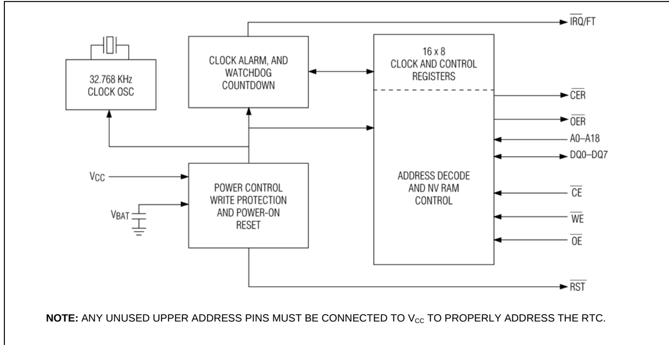
Figure 1. BLOCK DIAGRAM
