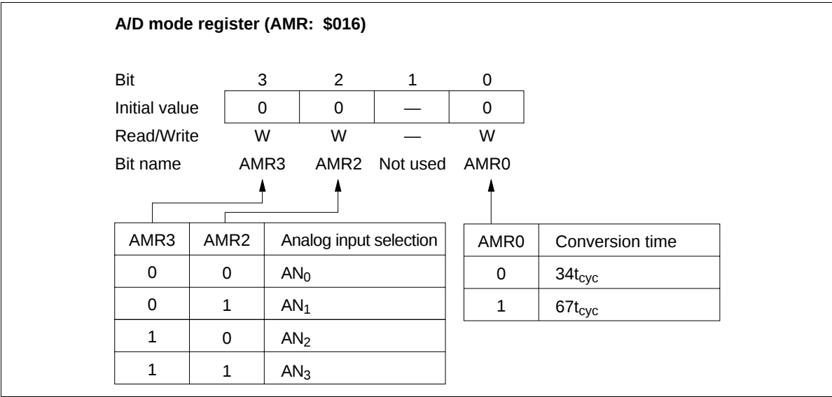
Figure 82 A/D Mode Register (AMR)
