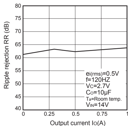
Fig.15 Ripple Rejection vs. Output Current (PQ120DNA1ZPH)
