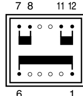
Primary winding
