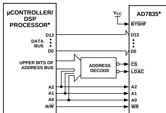
Figure 25. AD7835 16-Bit Interface
