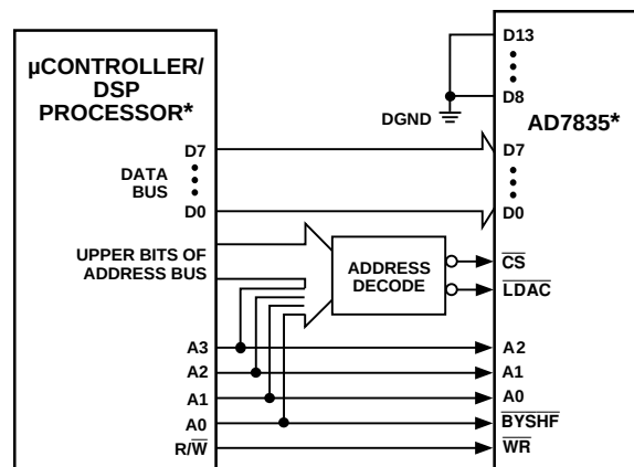
Figure 26. AD7835 8-Bit Interface
