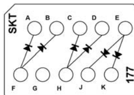
CTJ420E177 Six JANTX 1N4454-1 Diodes
