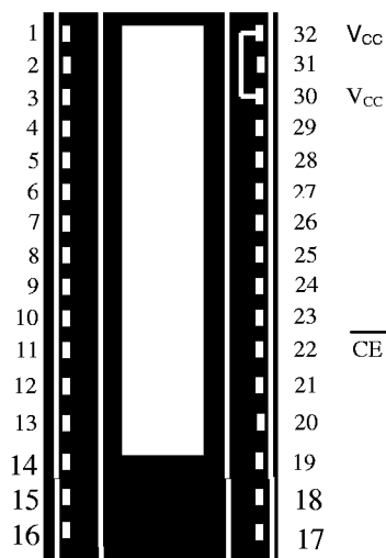
32-Pin Intelligent Socket
