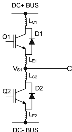
Figure 15: Parasitic Elements
