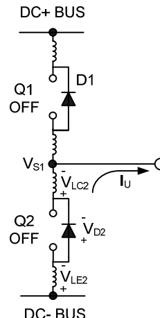
Figure 17: V_S negative
