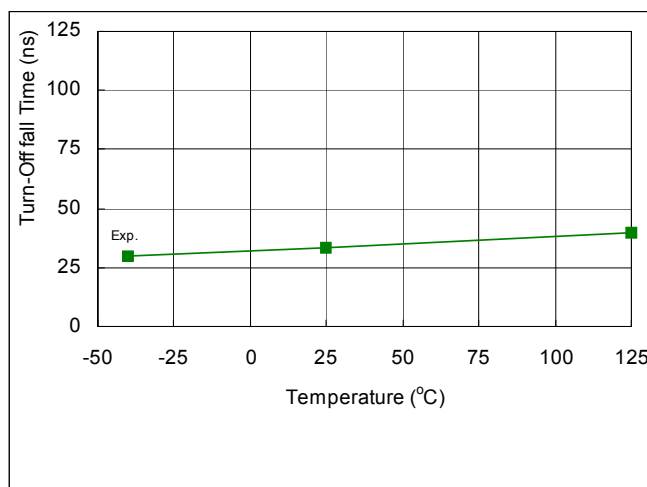
Fig. 27. Turn-off Rise Time vs. Temperature
