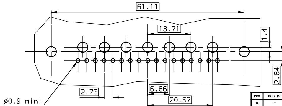
LAYOUT DIMENSIONS (after plating) CONNECTOR SIDE VIEW
