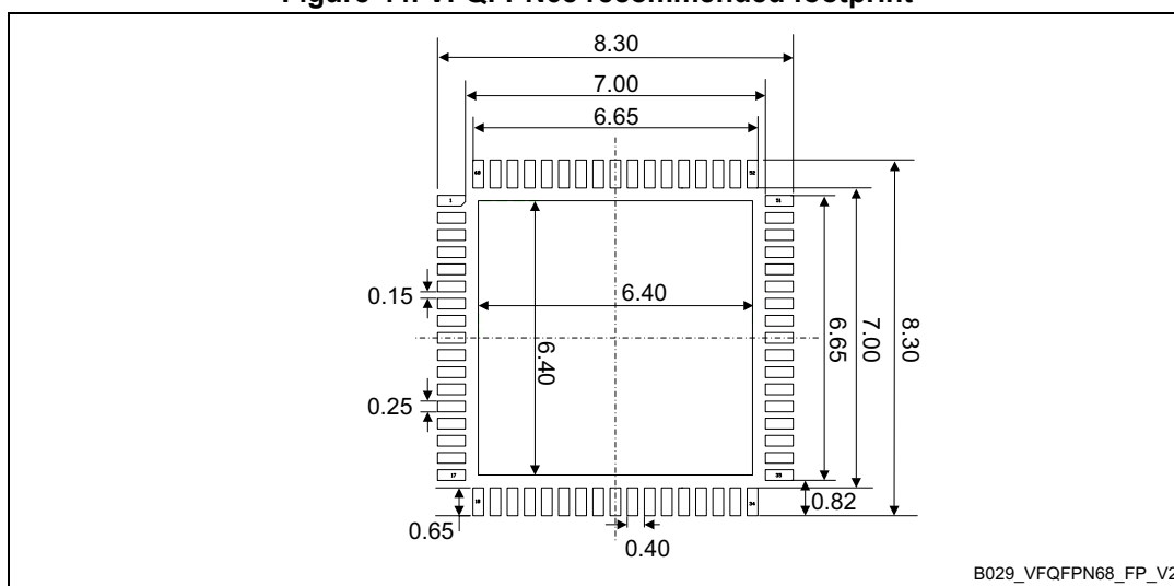
Figure 44. VFQFPN68 recommended footprint
