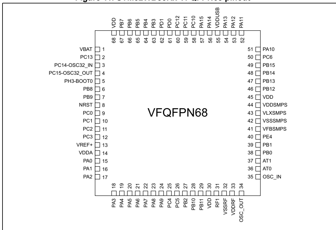
Figure 11. STM32WB55Rx VFQFPN68 pinout (1)(2)
