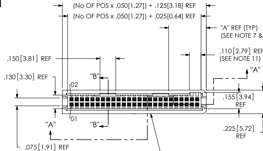
FIG 1 -01: THROUGH HOLE
