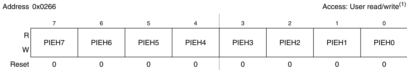
Figure 2-57. Port H Interrupt Enable Register (PIEH)
