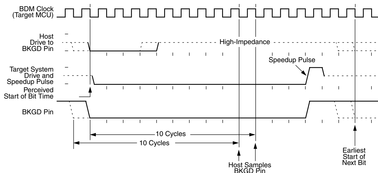
Figure 7-10. BDM Target-to-Host Serial Bit Timing (Logic 0)
