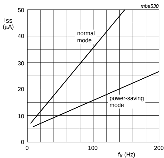
Fig 23. I_{SS} as a function of f_{fr}
