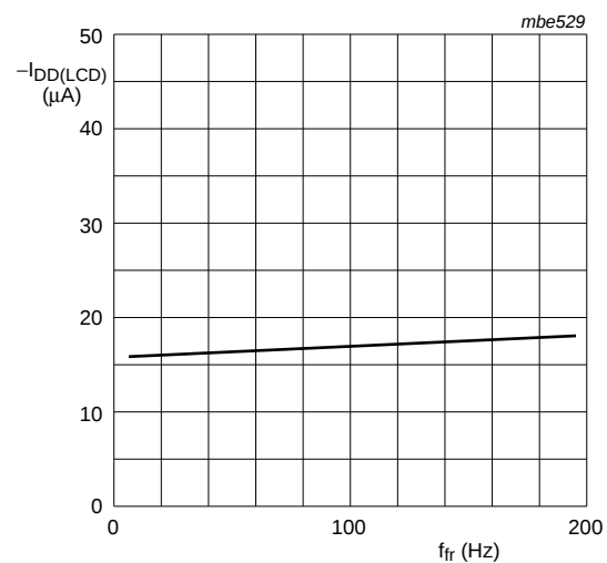
Fig 24. -I_{DD(LCD)} as a function of f_{fr}
