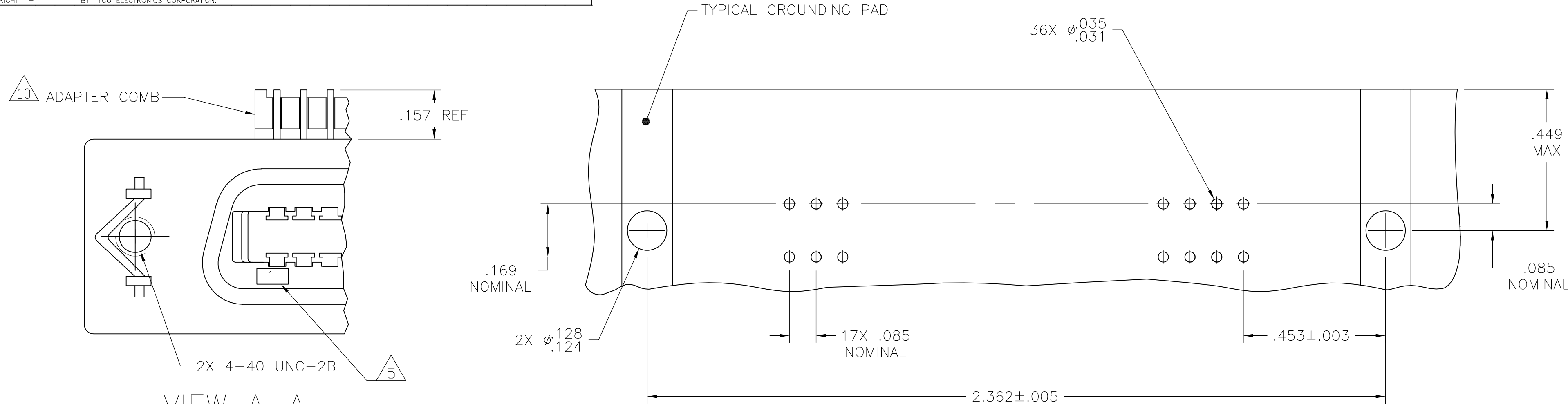
SUGGESTED PRINTED CIRCUIT BOARD MOUNTING DIMENSIONS
