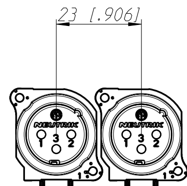
Layout tolerance: \pm 0.05\text{mm} [0.002"]
