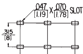
RECOMMENDED PC BOARD LAYOUT (Component Side)
