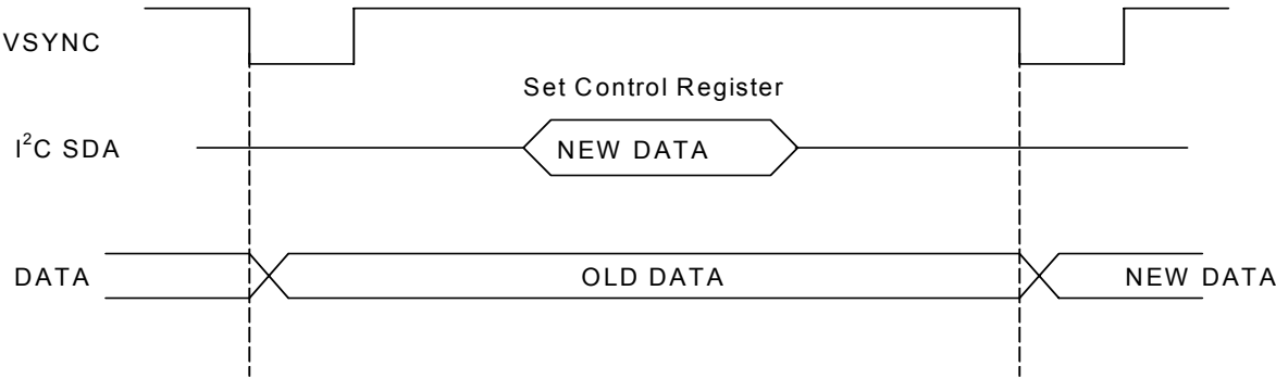
Fig. 8 WSS Data Renewal Timing
