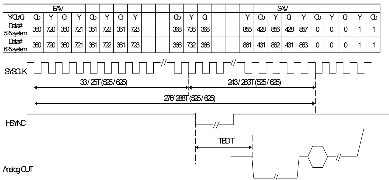
Fig. 10 Interface Timing (ITU-R BT.656 or Master mode)
