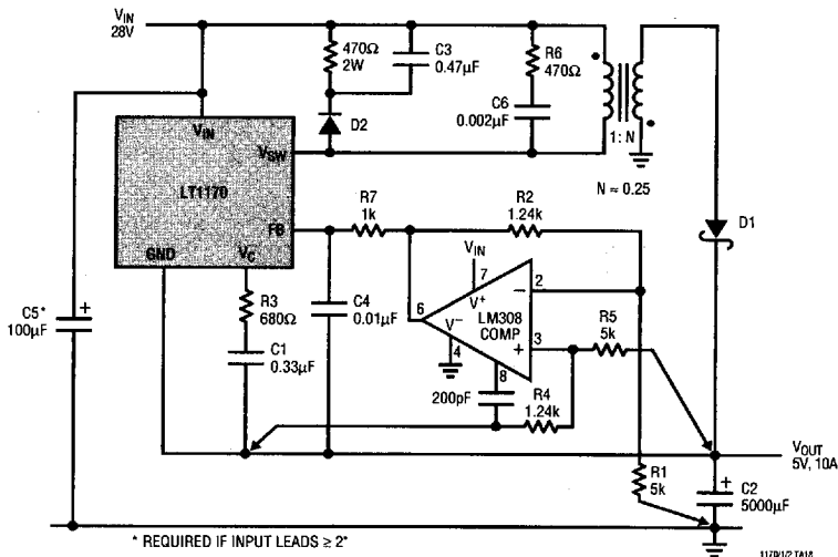
Positive Current Boosted Buck Converter
