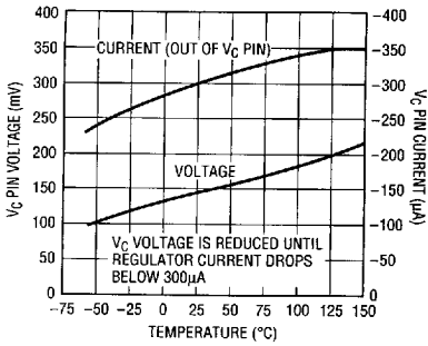
Shutdown Thresholds
