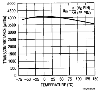
Error Amplifier Transconductance
