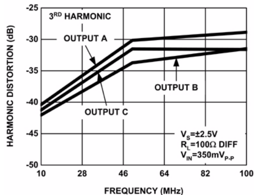
FIGURE 32. HARMONIC DISTORTION
