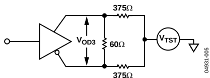
Figure 5. Driver Voltage Measurement over Common-Mode Voltage Range
