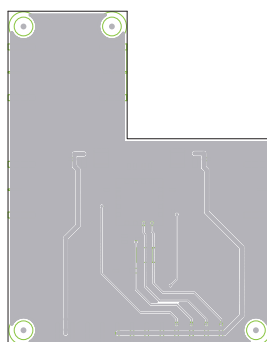
Layer 3: Signal
