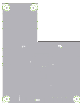
Layer 2: Ground
