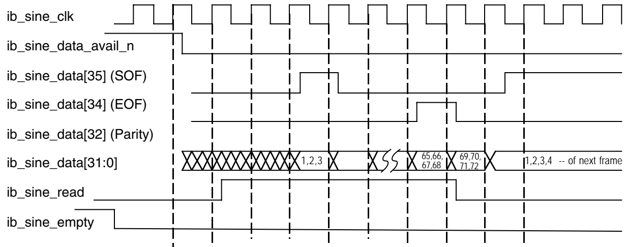
Figure 6. Inbound Generic FIFO Bridge Read Transfer (First Read After Empty)
