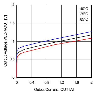
Fig.18 High side body diode (2A class)
