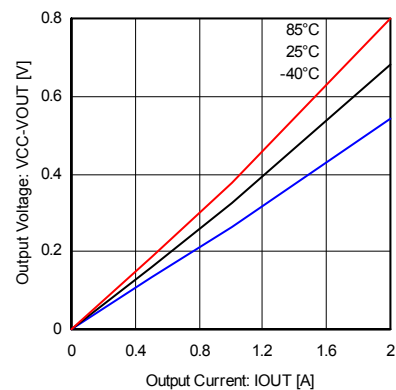
Fig.15 Output high voltage (2A class)
