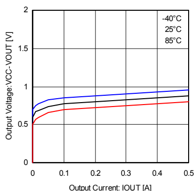
Fig.16 High side body diode (0.5A class)
