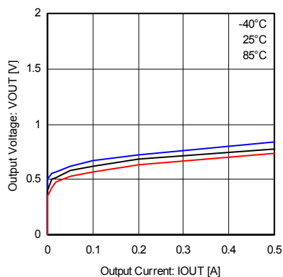
Fig.22 Low side body diode (0.5A class)
