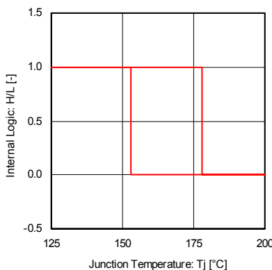
Fig.10 Thermal shutdown
