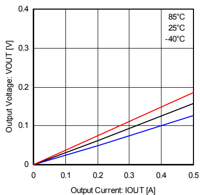
Fig.19 Output low voltage (0.5A class)
