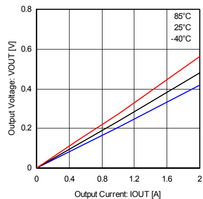
Fig.21 Output low voltage (2A class)
