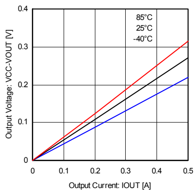
Fig.13 Output high voltage (0.5A class)
