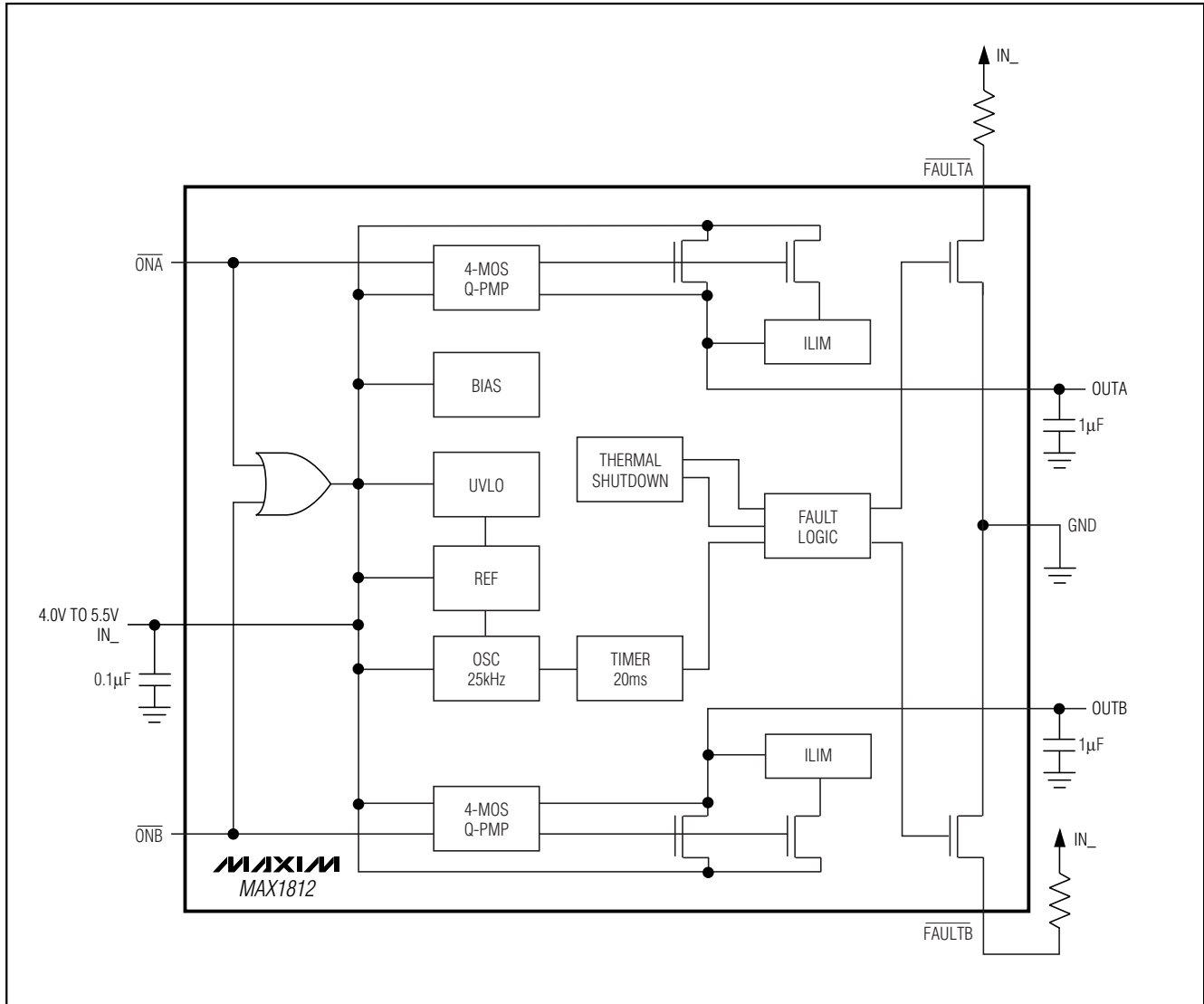
Figure 1. Functional Diagram
