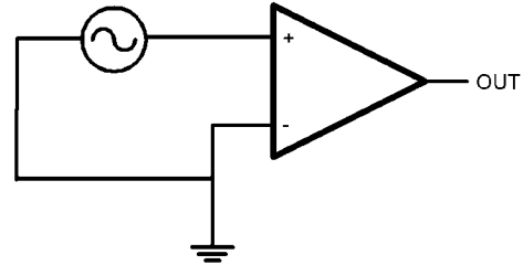
FIGURE 3. Zero-Crossing Detector
