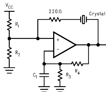
FIGURE 5. Crystal Oscillator
