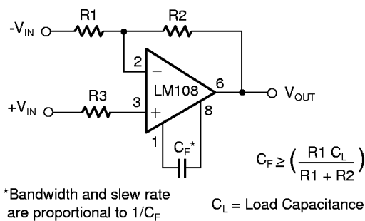
Figure 2. Standard Compensation Circuit
