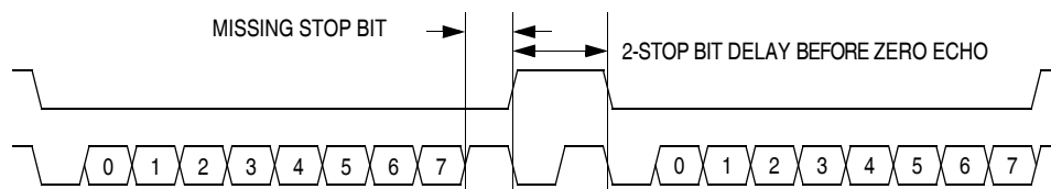
Figure 19-14. Break Transaction
