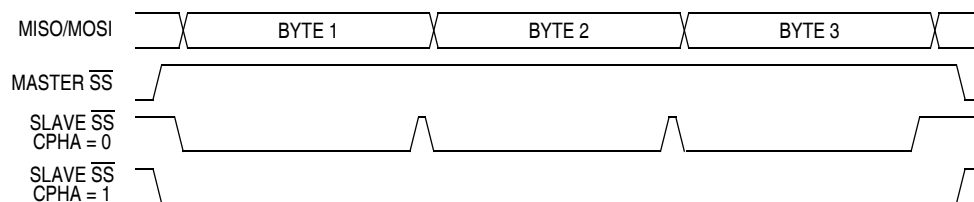
Figure 16-6. CPHA/SS Timing
