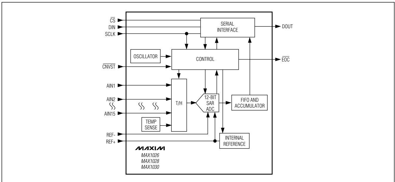
Figure 2. Functional Diagram
