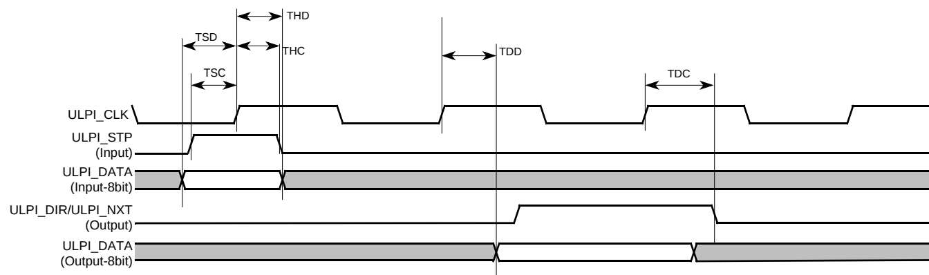
Figure 19. ULPI Timing Diagram
