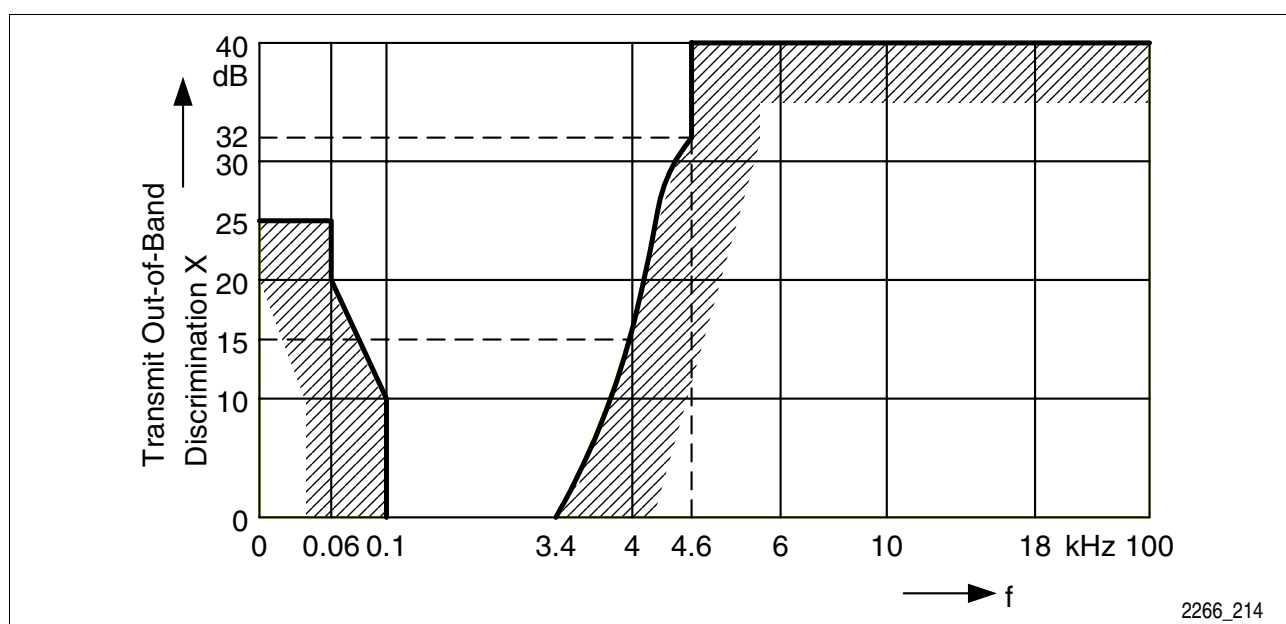
Figure 13 Out-of-Band Discrimination in Transmit Direction
