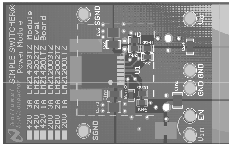
Figure 32. EVM Board Layout - Top View
