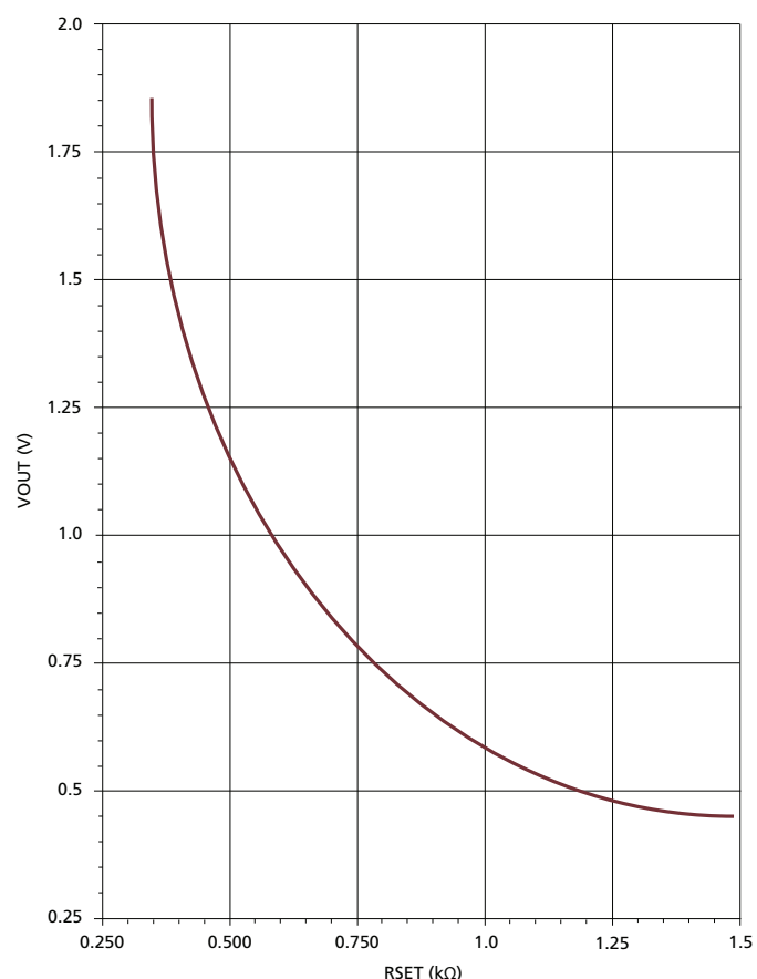
Figure 4-1: V_{\text{OUT}} vs. RSET
