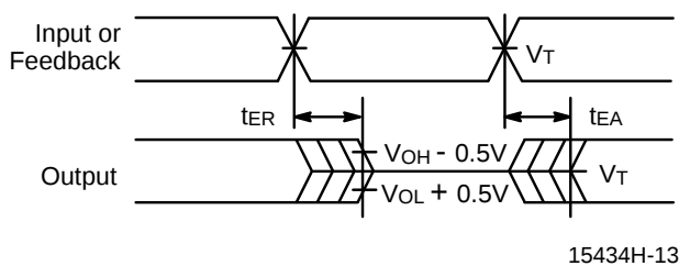
Input to Output Disable/Enable
