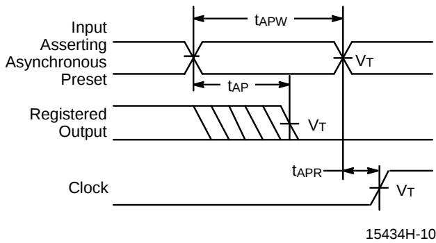
Asynchronous Preset
