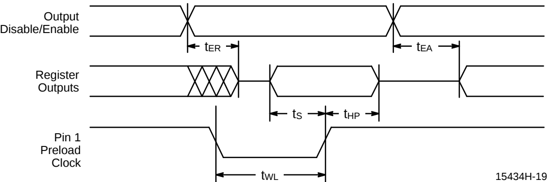
Output Register Preload Waveform
