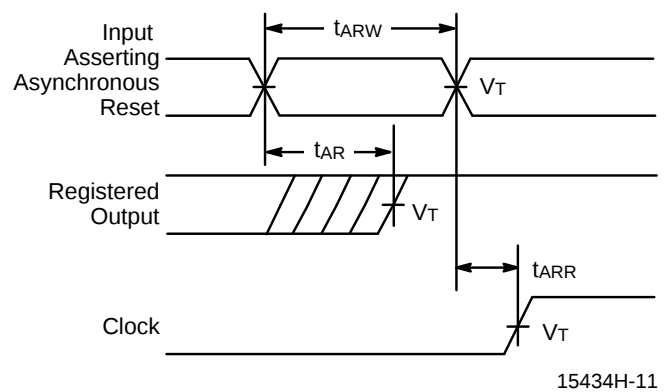
Asynchronous Reset
