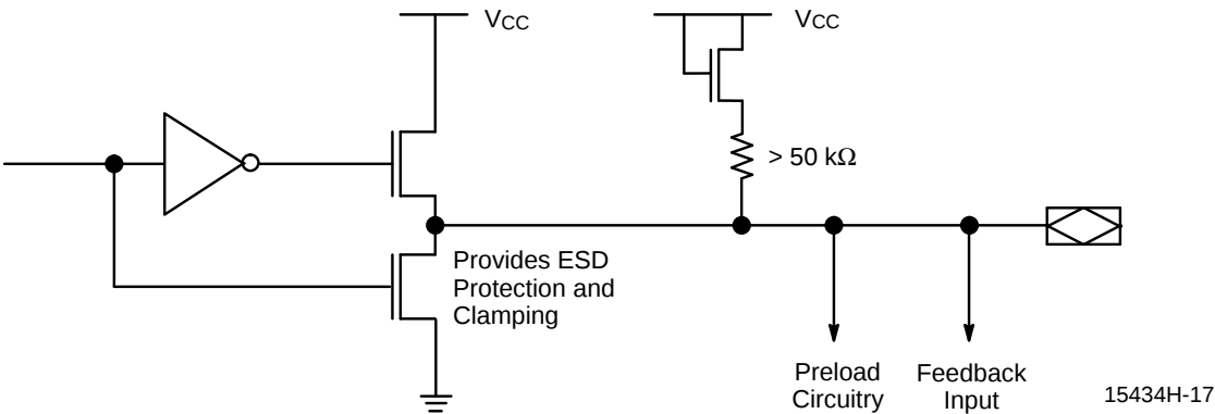
Typical Output
