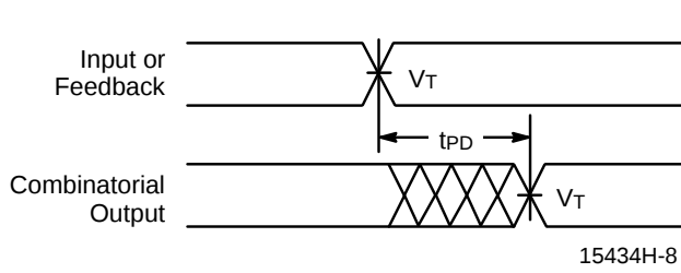
Combinatorial Output
