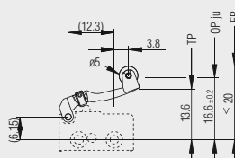
L43: adjustable roller lever 190.072.013
