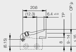
L41: adjustable plastic lever 190.075.013
