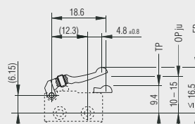
L45: adjustable simulated roller 190.074.013
