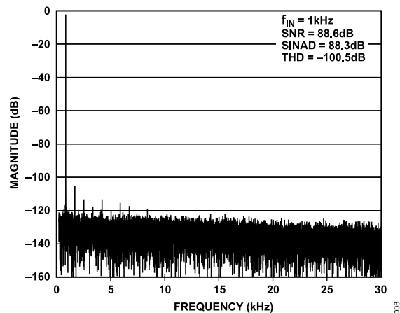
Figure 11. Typical Fast Fourier Transform (FFT)
