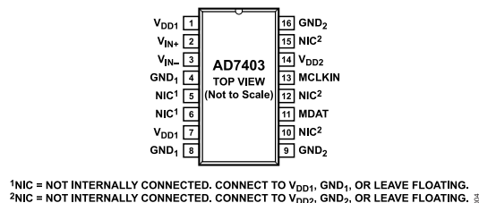
Figure 5. AD7403 Pin Configuration
