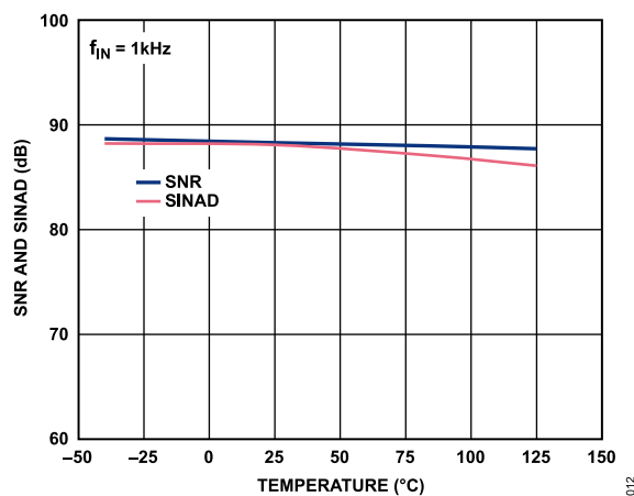
Figure 16. SNR and SINAD vs. Temperature
