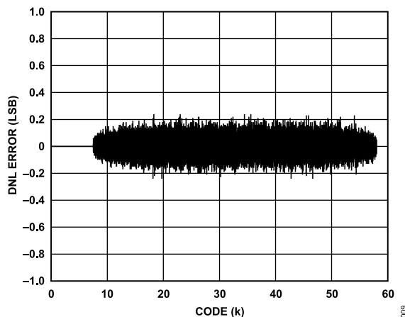
Figure 12. Typical DNL Error
