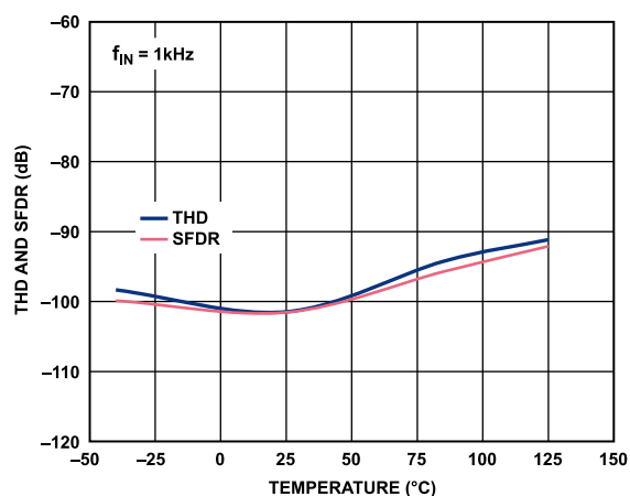
Figure 17. AD7403 THD and SFDR vs. Temperature
