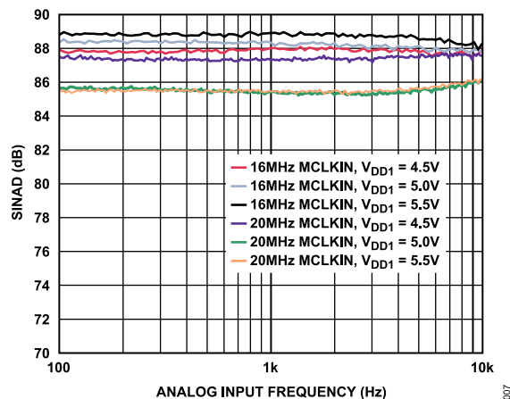
Figure 10. SINAD vs. Analog Input Frequency
