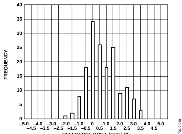
Figure 13. AD5380-REFOUT Temperature Coefficient
