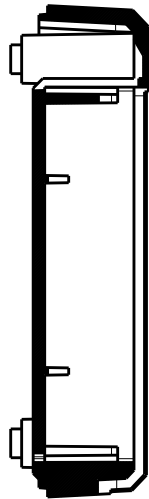
SECTION J-J
