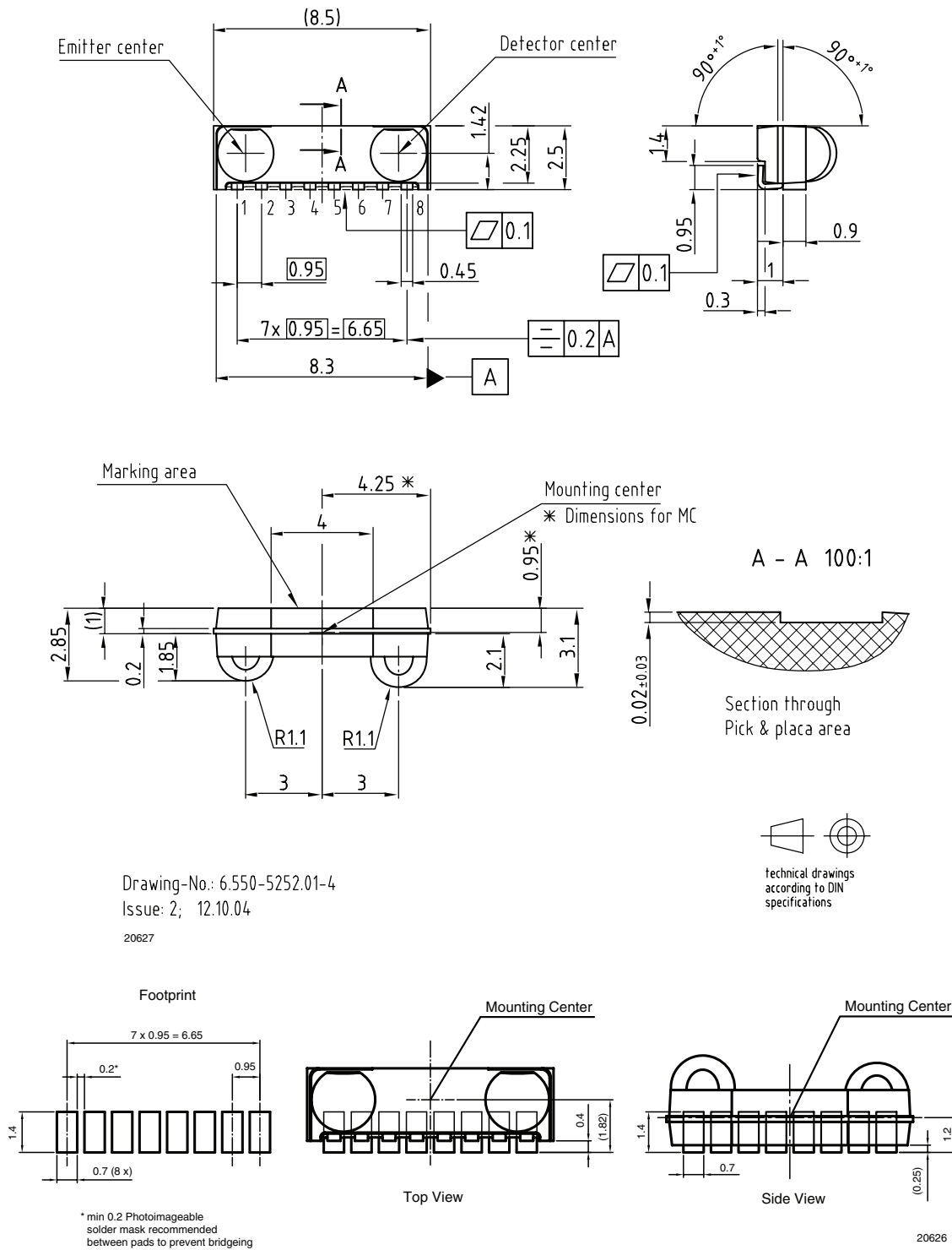
Figure 8. Package Drawing
