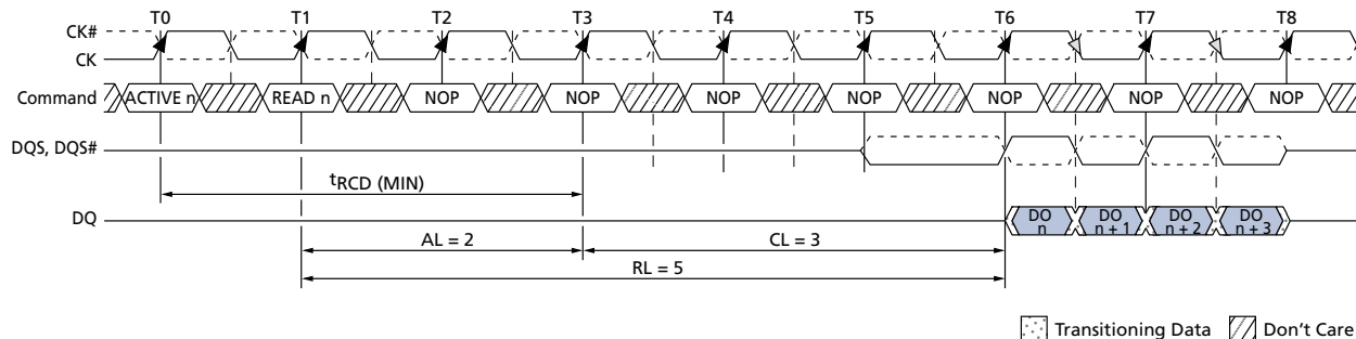
Figure 39: READ Latency
