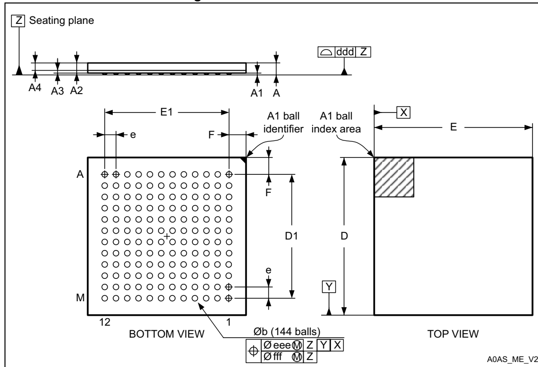
Figure 90. UFBGA144 outline
