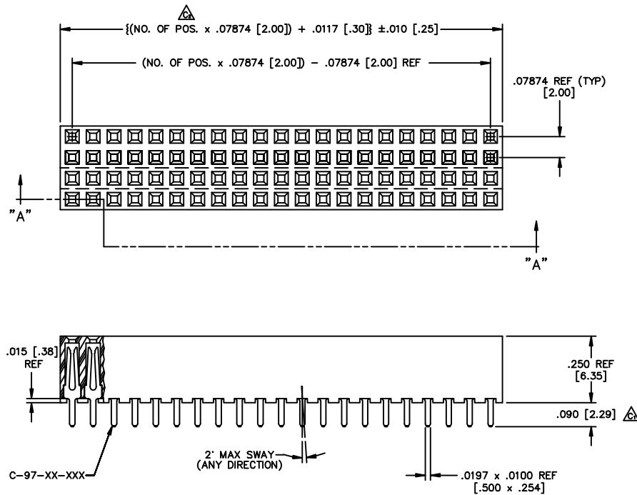
SECT. "A-A"
