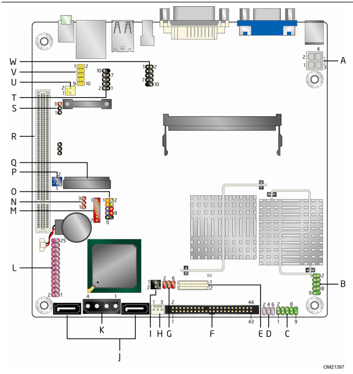
Figure 2-4. Component-side Connectors and Headers
