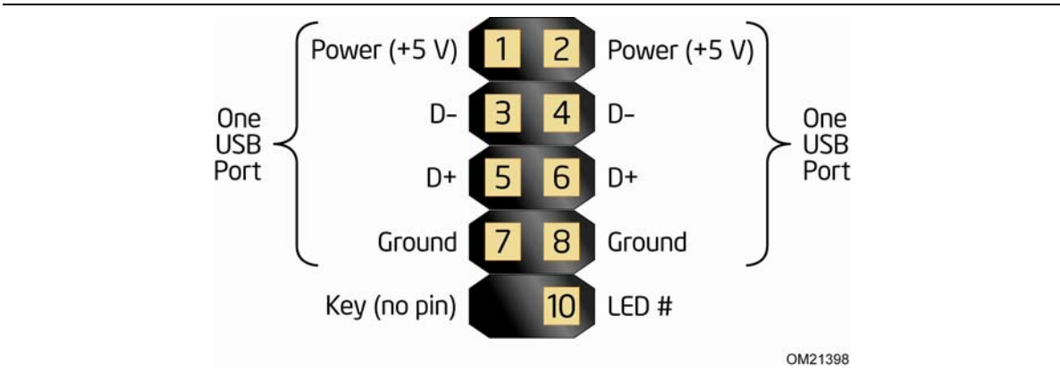
Figure 2-7. Connection Diagram for Front Panel USB Header (with Intel Z-U130 USB Solid-State Drive, or Compatible Device, Support)
