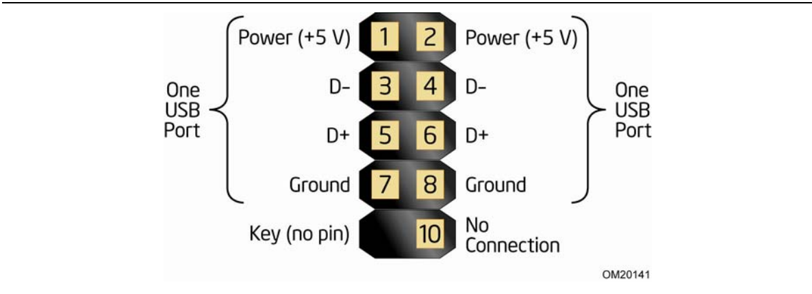
Figure 2-6. Connection Diagram for Front Panel USB Header
