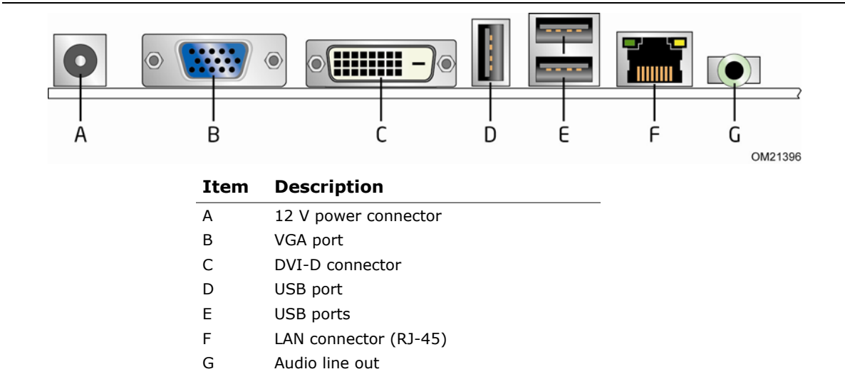
Figure 2-2. Back Panel Connectors
