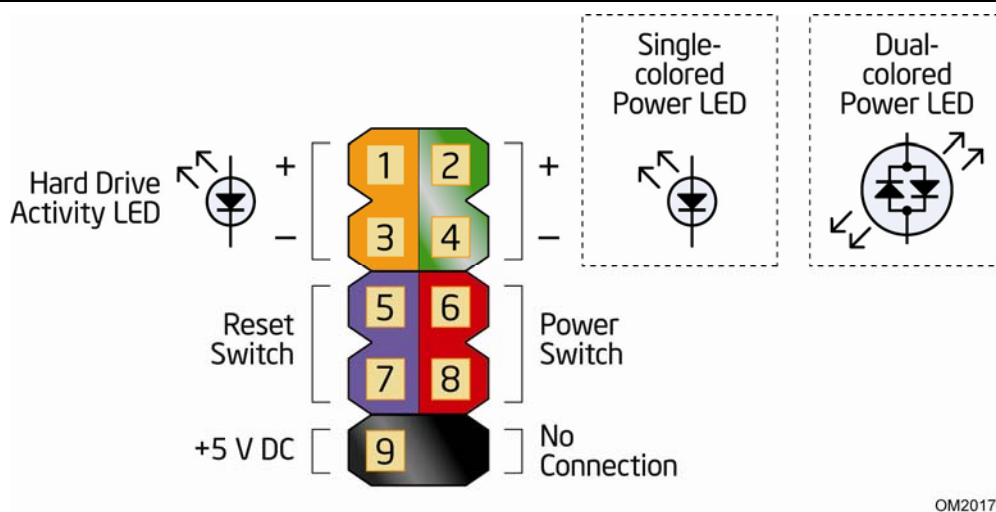
Figure 2-5. Connection Diagram for Front Panel Header
