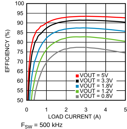
Figure 4. Efficiency with P_{VIN} = A_{VIN} = 12\text{ V}
