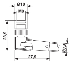
Dimensional drawing
