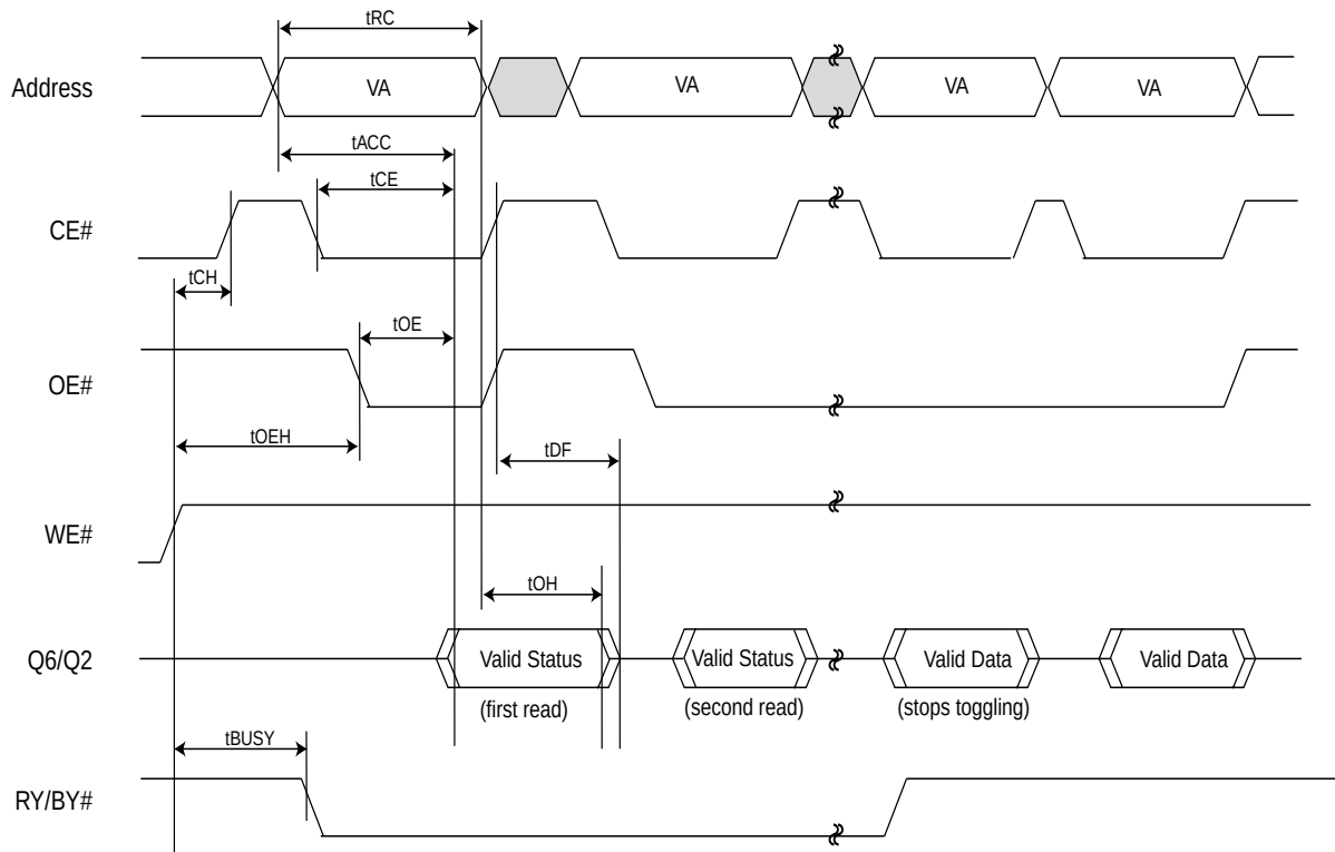
Figure 20. TOGGLE BIT TIMING WAVEFORMS (DURING AUTOMATIC ALGORITHMS)
