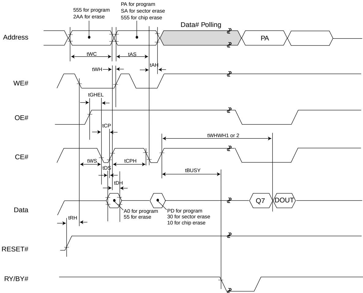
Figure 11. CE# CONTROLLED WRITE TIMING WAVEFORM
