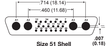
Size 51 Shell 20 Micro contacts 4 Coax or 4 Power (Not MS) 25P4 25C4
