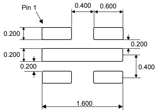
Figure 17. UFDFPN5 - Footprint example
