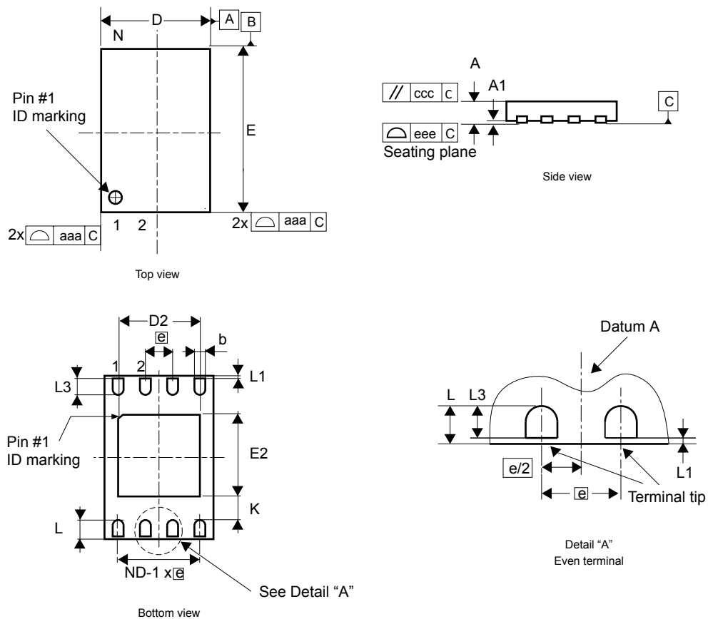
Figure 18. UFDFPN8 - Outline
