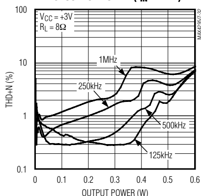
MAX4297 TOTAL HARMONIC DISTORTION PLUS NOISE vs. OUTPUT POWER ( f_{IN} = 20kHz )
