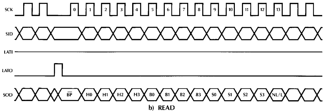
Figure 6. Serial Timing
